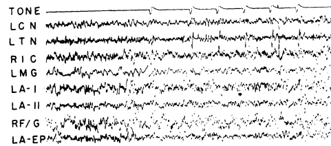
Figure 4: Trial 13 (begins to wait for tones)
