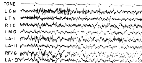
Figure 3: Trial 1 (no behavioral evidence of learning)
